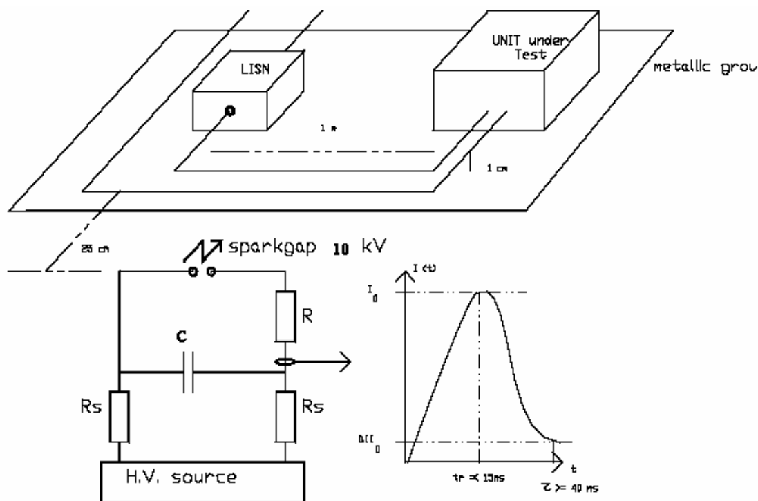
Figure 34 ESD Radiated Discharge Test Set-up
