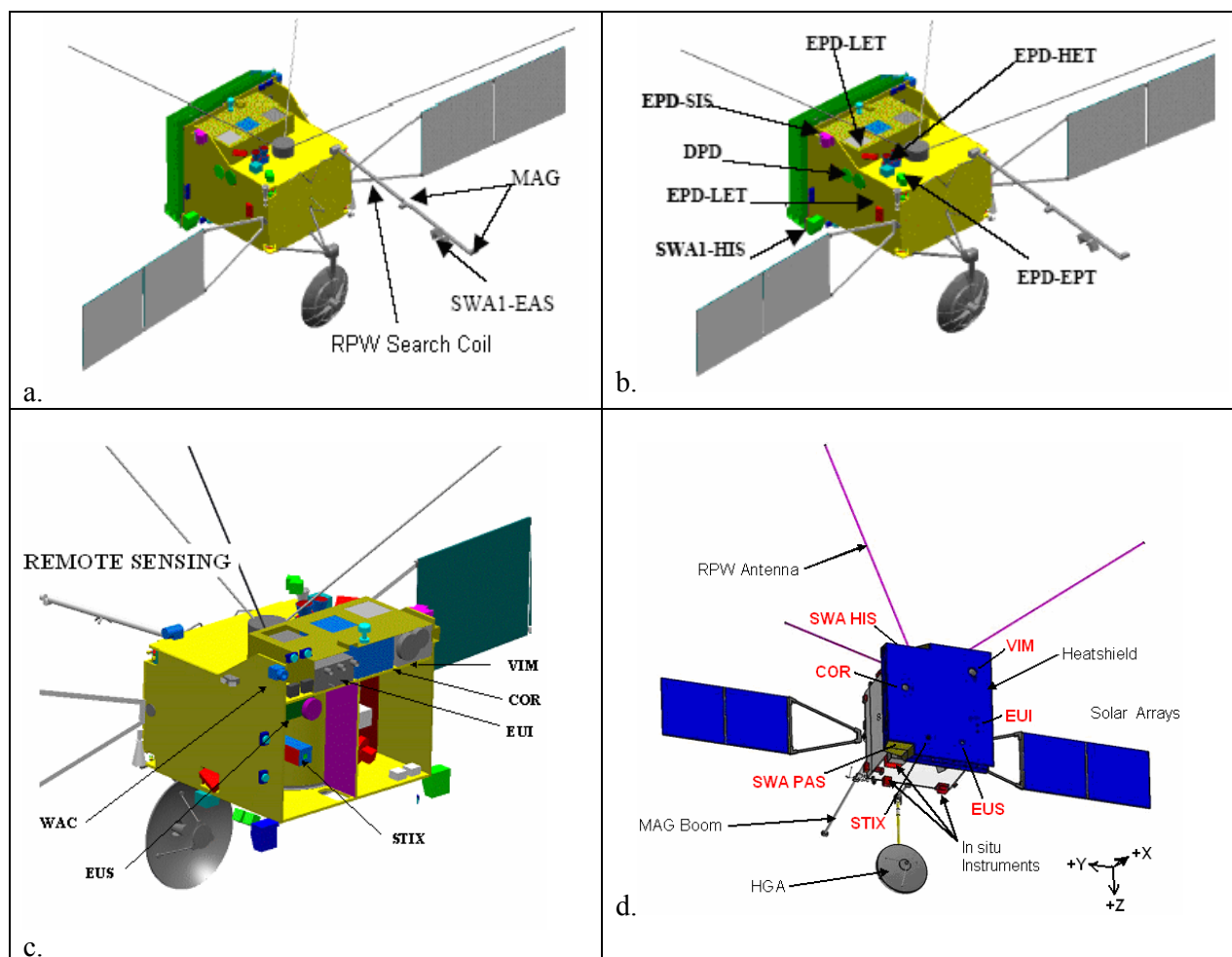
Figure 3 Preliminary Instrument Accommodation Concepts
