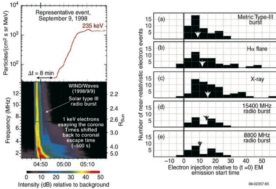
Figure 2-11 Systematic delays between electromagnetic emissions and interplanetary near-relativistic electrons. The left panel shows a representative event in which the onset of >200 \text{ keV} electrons is delayed with respect to the start of type III radio emission by \sim 8 \text{ min} . Are these delays due to the acceleration process, or are they controlled by the particle escape onto interplanetary magnetic field lines?
