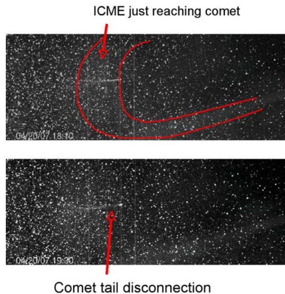
Figure 2-13 Two images from the Heliospheric Imager on STEREO showing the dislocation of the tail of Comet Encke as the result of the passage of an ICME. In-situ measurements of the ICME's magnetic field and plasma properties from multiple spacecraft near the location of the comet would have provided invaluable information about CME structure and evolution.
