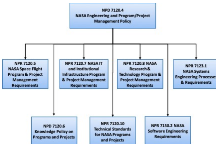
Figure 1-2 - Documentation Relationships
