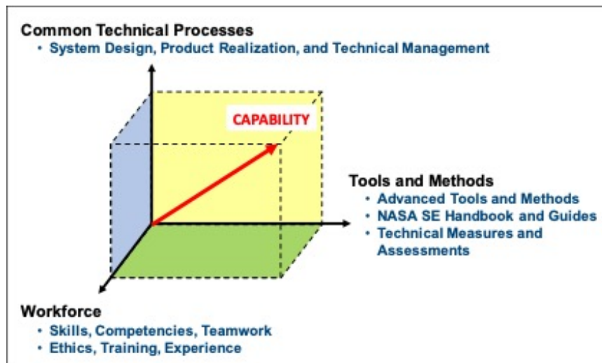
Figure 1 4 - SE Framework
